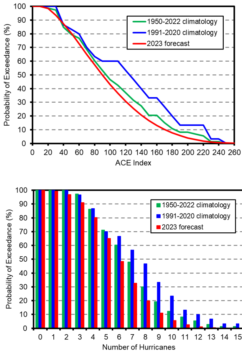
Figure 1. Forecast probability of exceedance (PoE) plots for the North Atlantic ACE index in 2023 (upper panel) and for the number of North Atlantic hurricanes in 2023 (lower panel). Each plot displays three sets of PoE data comprising the TSR forecast PoE curve issued pre-season and two climatology PoE curves.
