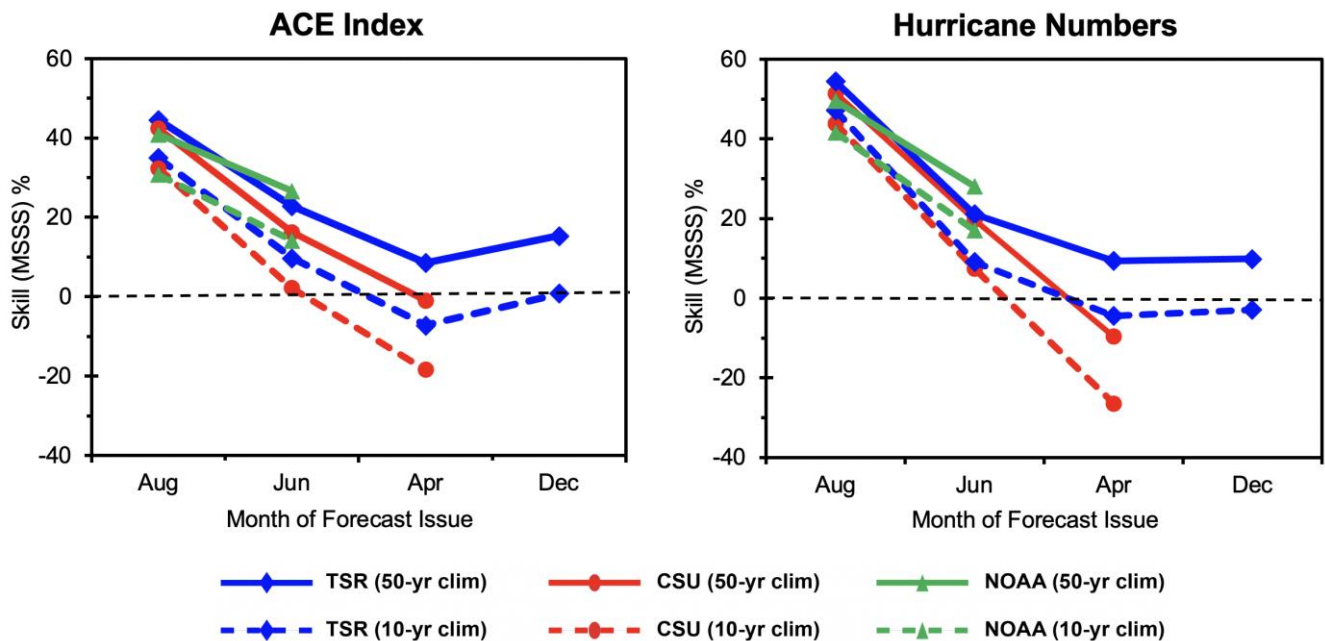
Figure 3. Real-time skill of North Atlantic seasonal tropical cyclone outlooks assessed for the 19-year period 2003-2021. The skill of the seasonal outlooks issued publicly by Tropical Storm Risk (TSR, blue lines), Colorado State University (CSU, red lines), and the National Oceanic and Atmospheric Administration (NOAA, green lines) are compared for ACE (left panel) and for hurricane numbers (right panel). The skill is shown as the Mean Square Skill Score (MSSS) based on a fixed 50-year (1951-2000) climatology and on a running prior 10-year climate norm.
