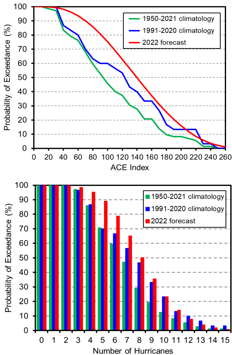
Figure 1. Forecast probability of exceedance (PoE) plots for the North Atlantic ACE index in 2022 (upper panel) and for the number of North Atlantic hurricanes in 2022 (lower panel). Each plot displays three sets of PoE data comprising the TSR forecast PoE curve issued in early April and two climatology PoE curves.
