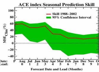
Figure 9. Simulated real time forecast skill for the period 1988-2002 for the northwest Pacific ACE index.
