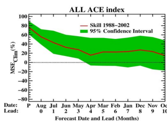
Figure 4. Simulated real time forecast skill for the period 1988-2002 for the Atlantic total ACE index.
