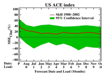
Figure 6. Simulated real time forecast skill for the period 1988-2002 for the US landfalling ACE index.
