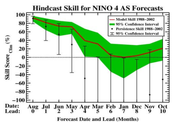
Figure 8. Simulated real time forecast skill for the period 1988-2002 for the Niño 4 SST region.
